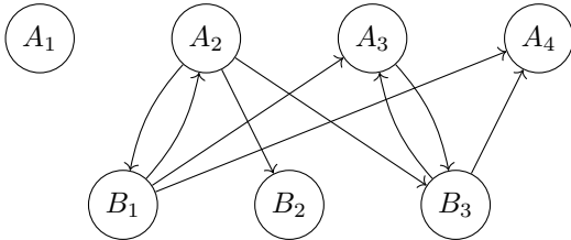
Fig. 1. Graphical representation of \mathcal{AF}(\text{AT}_2) .
