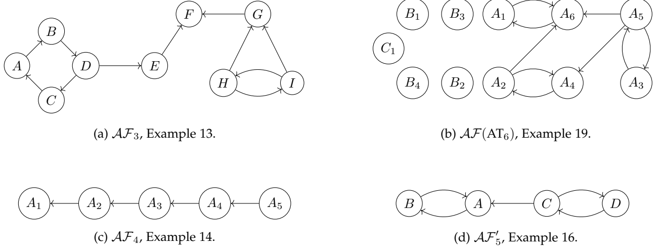
Fig. 2. Graphical representations of the AFs in Section 4.
